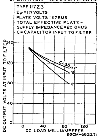
OPERATION CHARACTERISTICS
