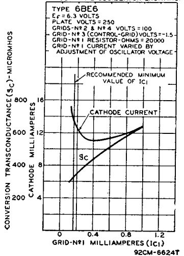
OPERATION CHARACTERISTICS WITH SEPARATE OSCILLATOR EXCITATION
